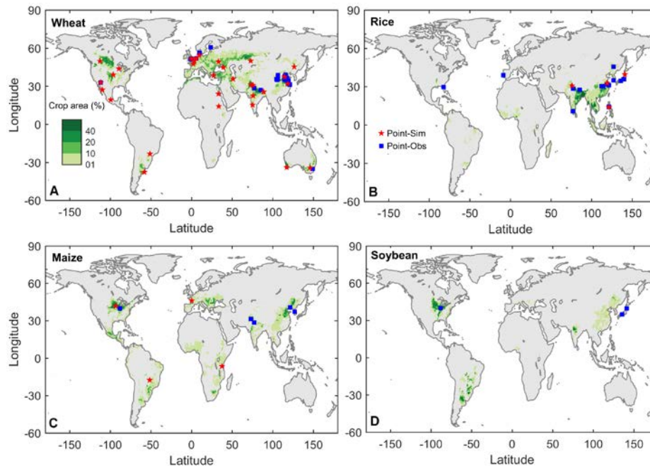
Figure S1. Maps of study sites for point-based model-ensemble simulations and field warming experiments that focused on the warming impacts on yields of four crops. For simulation experiments, only multi-model results were used (i.e. no single model applications were included here). Crop-growing area data from Monfreda et al. 2008 (29) is shown by green shading. For model-ensemble simulations, there are in total 30 sites for wheat, 4 for rice, and 4 for maize. For field warming experiments, there are in total 25 experimental sites for wheat, 15 for rice, 5 for maize and 3 for soybean.
