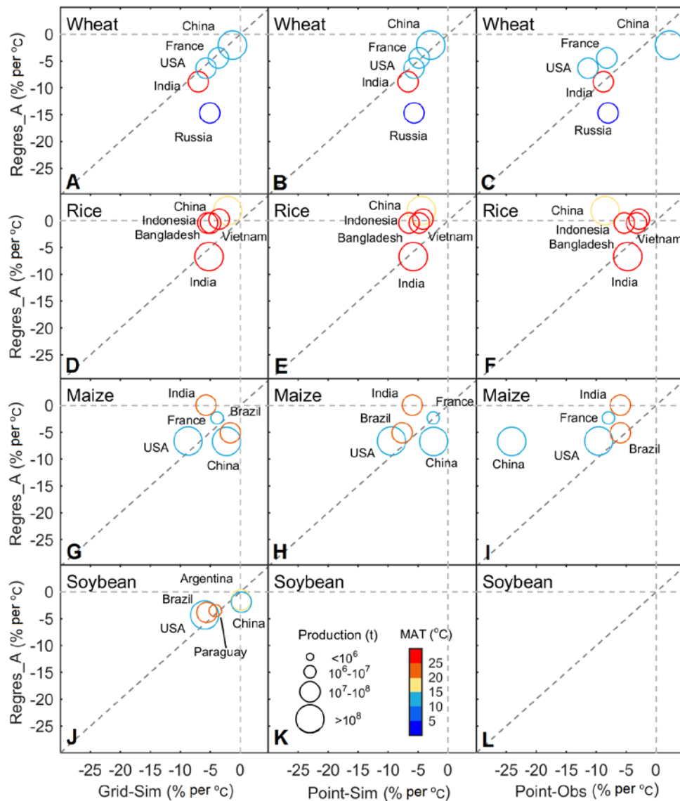
Figure S3. Comparison of estimates of +1 °C global temperature impacts on yields from Grid-Sim, Point-Sim and Point-Obs with Regres_A methods for the five major countries producing each crop (10). The size of circles represents the country's annual crop production (15). The color of circles represents the baseline (1981-2010) mean annual temperature (MAT) for each country's crop growing area (AgCFSR; http://data.giss.nasa.gov/impacts/agmipcf/ ).
