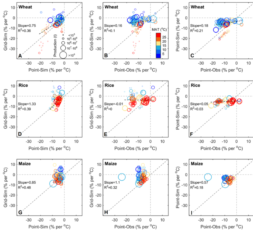
Figure S2. Country-scale pairwise comparisons of Grid-Sim, Point-Sim and Point-Obs method estimates of +1 °C global temperature impact on crop yield. The size of the circles is proportional to the country's annual crop productions (FAO, 2014). The color of circles represents the baseline (1981-2010) mean annual temperature (MAT) for each country's crop growing area (AgCFSR; http://data.giss.nasa.gov/impacts/agmipcf/ ). The weighted linear regressions were used to explore the relationship between different methods with weighting factors for each country's production. For maize, the observed data from China (outlier) was not included in the regression.
