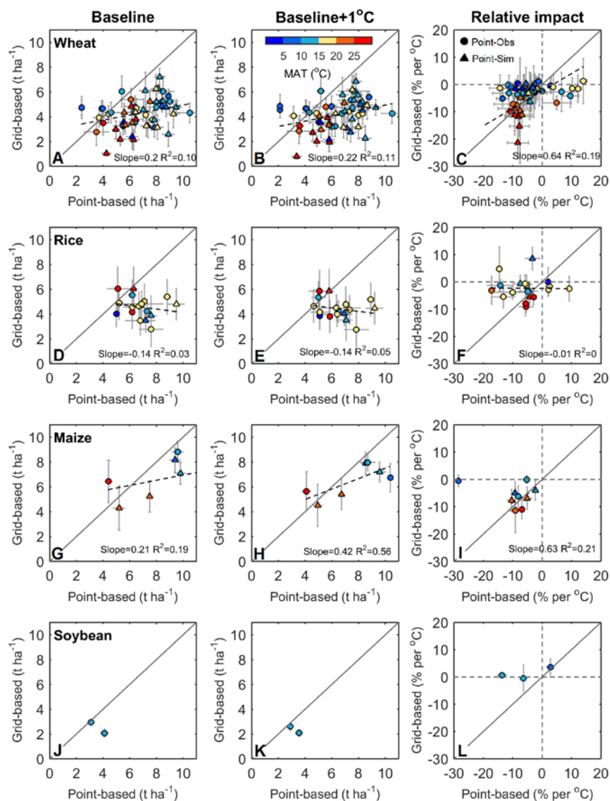
Figure S4. Site-scale estimates of +1 °C global temperature impact from Grid-Sim compared with Point-Sim and Point-Obs methods. The comparisons include absolute yield impacts for periods of baseline (1981-2010) and baseline+1 °C global temperature and relative yield change. Note, more relative impact observations were available than absolute impact. The color of symbols represents baseline mean annual temperature (MAT; AgCFSR; http://data.giss.nasa.gov/impacts/agmipcf/ ). Triangles and circles represent point-based model-ensemble simulation and field warming experiment, respectively. Linear regressions were used to explore the relationship between point-based and grid-based methods. For maize, the observed data from China (outlier) was not included in the regression.
