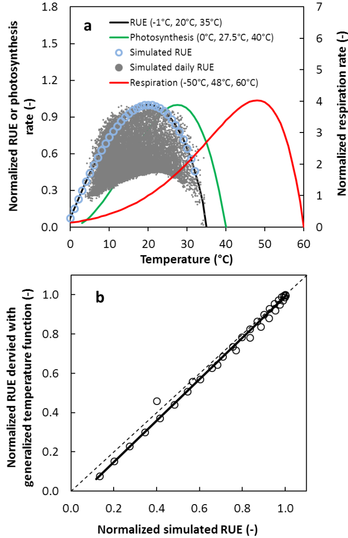
Supplementary Figure 2 | Radiation use efficiency (RUE) temperature dependency derived from photosynthesis and respiration. (a) RUE temperature response functions averaged under low (10 MJ m -2 d -1 ; circles) and high (30 MJ m -2 d -1 ; blue circles) conditions, and RUE under various (grey dots) radiation conditions calculated with the SPASS photosynthesis and plant growth model 69 . Red and green solid lines are the derived temperature response functions for photosynthesis and respiration rates used in SPASS to calculate daily RUE, respectively. The temperature responses for photosynthesis (green line), respiration (red line), and RUE (black line) were produced using the cardinal temperatures shown in parenthesis with \beta = 1.0 for photosynthesis and respiration and 0.8 for RUE. The black line roughly captures the envelope of the simulated daily RUE response to temperature by the SPASS model. (b) Comparison of normalized RUE calculated using the derived temperature response function shown in (a) with mean daily RUE calculated using the SPASS model for temperatures ranging from 0°C to 32°C. Solid and dashed lines are the standardized linear regression ( y = -1.0556 [1.0305, 1.0814] x - 0.0643 [-0.0844, -0.0441] , r^2 = 0.99 , P < 2.22 \times 10^{-16} ) and the 1:1 line, respectively. All rates were normalized at 20°C.
