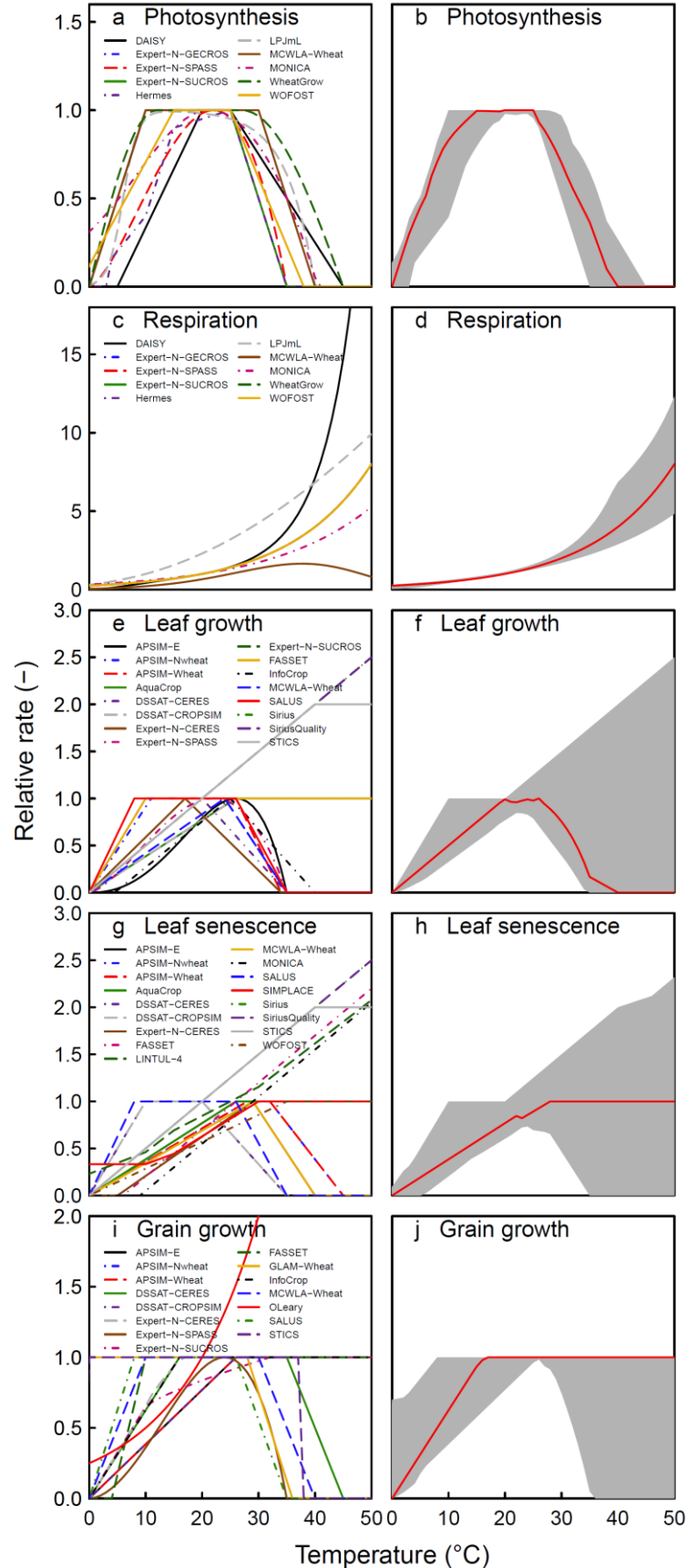
Supplementary Figure 1 | Temperature response functions in 29 wheat simulation models. (a and b) photosynthesis. (c and d) respiration. (e and f) leaf area growth. (g and senescence) senescence. Grain growth (i and j). Models are listed in Supplementary Table 1. (b, d, f, h, and j) Summaries of temperature responses from all models with red lines representing the median and shaded areas the 10% and 90% quantiles.
