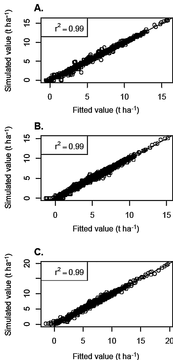
Fig. 1. Simulated values of maize (A), wheat (B), and rice (C) yields as a function of fitted values obtained with the selected statistical models. Each graphic includes yield data simulated in four sites.
