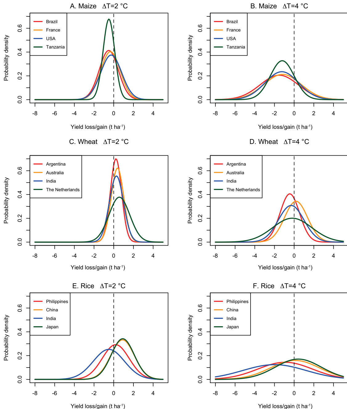
Fig. 4. Probability distributions of yield loss (or yield gain) resulting from an increase of temperature of +2^\circ\text{C} (A, C, E) or +4^\circ\text{C} (B, D, F) for maize, wheat, and rice (four sites per crop). The \text{CO}_2 concentration increase is set to +180 ppm in all cases ( [\text{CO}_2] = 570 ppm). Each distribution describes the variability of the yield loss (or gain) values simulated by different crop models.
